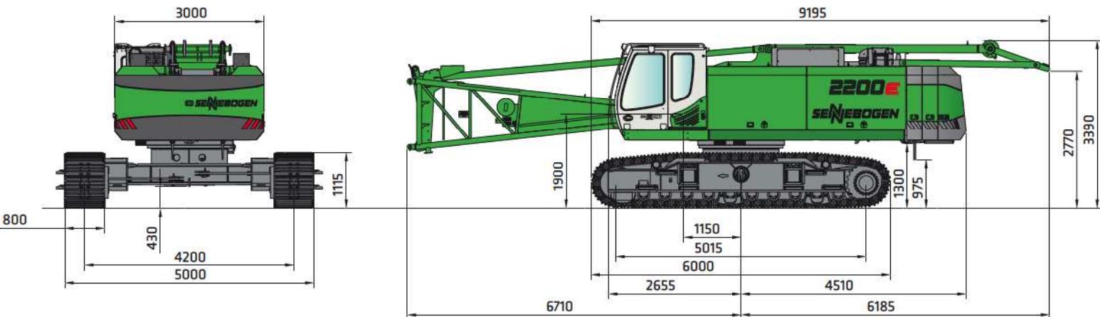
Grundmaschine base machine
